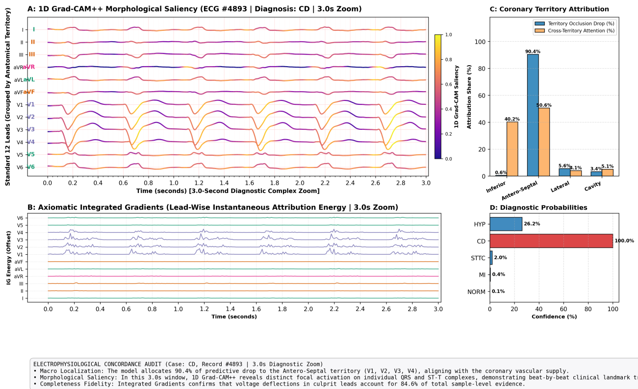
Figure 7: Multi-Scale Anatomical Attribution for Conduction Disturbance (CD, Record #4893). 1D Grad-CAM++ isolates the widened QRS complex and slurred intrinsicoid deflection in Antero-Septal leads ( \Delta P = 0.395 ).
